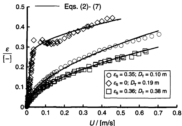
Figure 9. Test of experimental data for total gas holdup against the model predictions using Eqs. 2-7.
